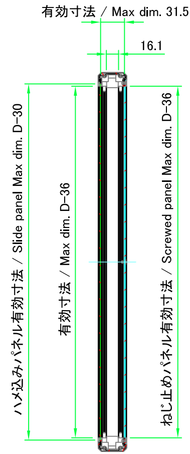
B-B (1:5)
